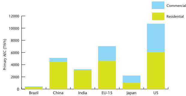
Figure 6: Primary energy (2003) 14
