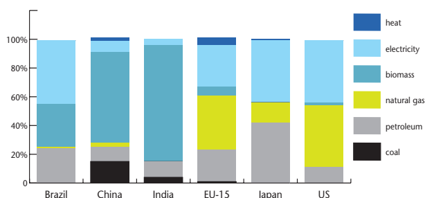
Figure 5: Site energy sources (2003) 13
