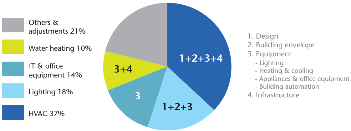
Figure 19: Design impacts on energy use 23
