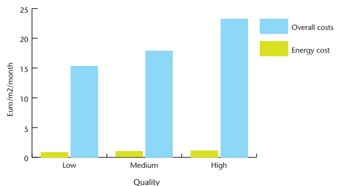
Figure 20: Energy and total costs by quality of fittings 25
